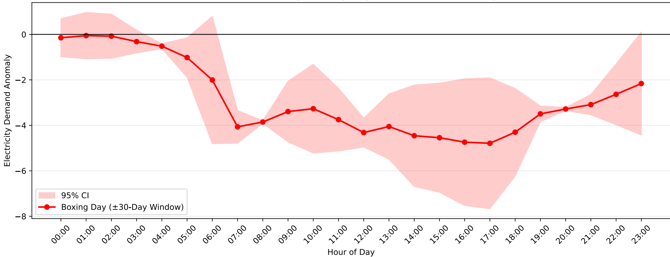
Mortdale Demand Anomaly: Boxing Day (2013-2014, \pm 30 -Day Window)
