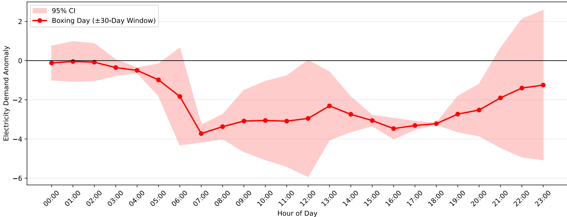
Mortdale Demand Anomaly: Boxing Day (2014–2015, \pm 30 -Day Window)
