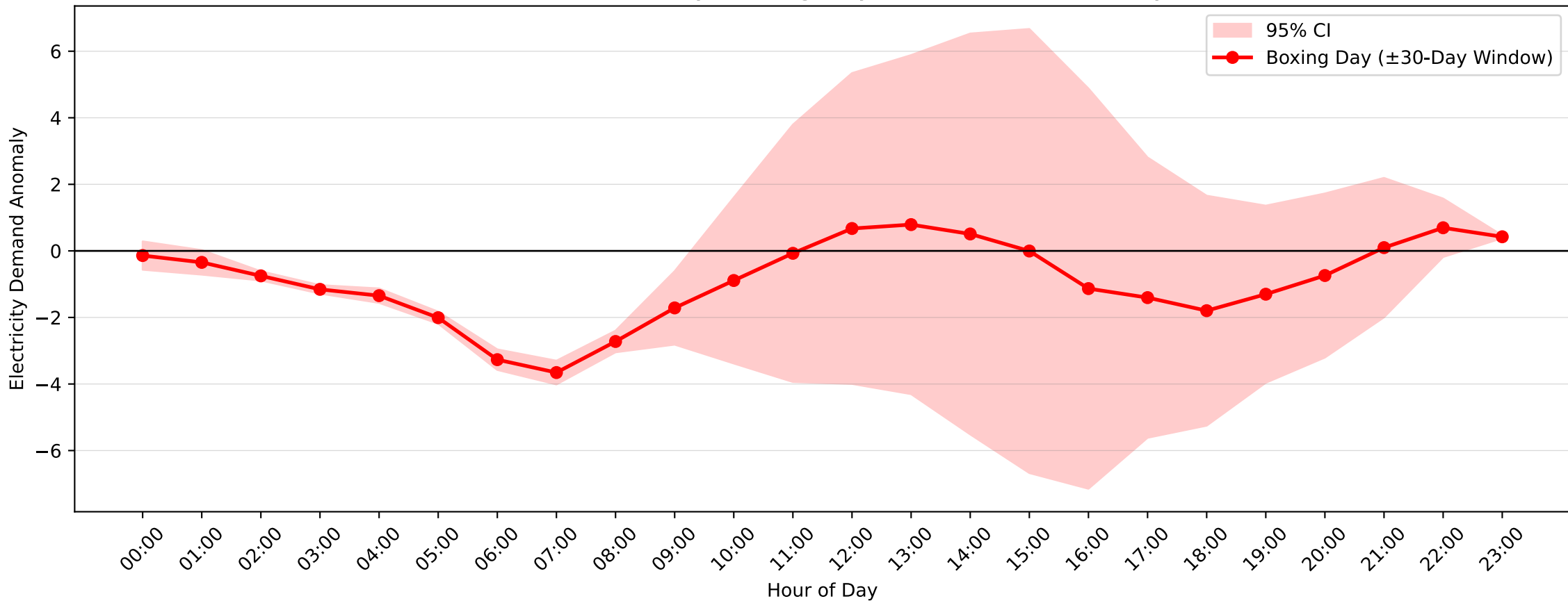
Mortdale Demand Anomaly: Boxing Day (2015–2016, \pm 30 -Day Window)
