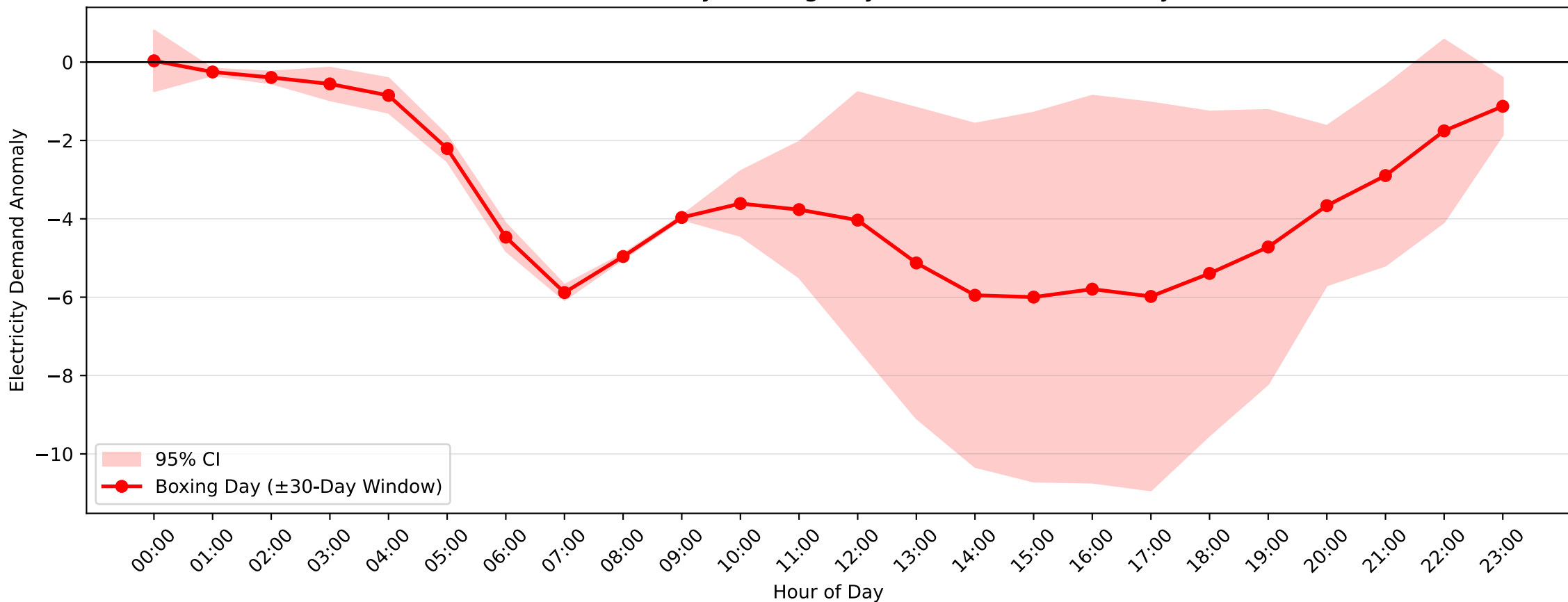
Mortdale Demand Anomaly: Boxing Day (2005–2006, \pm 30 -Day Window)
