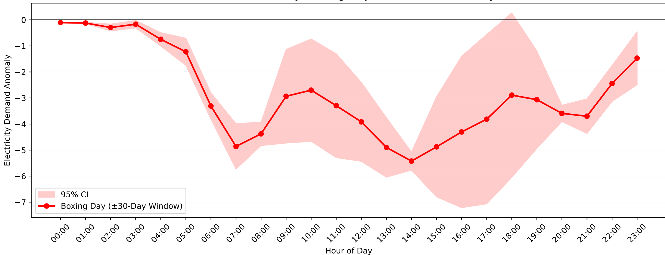
Mortdale Demand Anomaly: Boxing Day (2009–2010, \pm 30 -Day Window)
