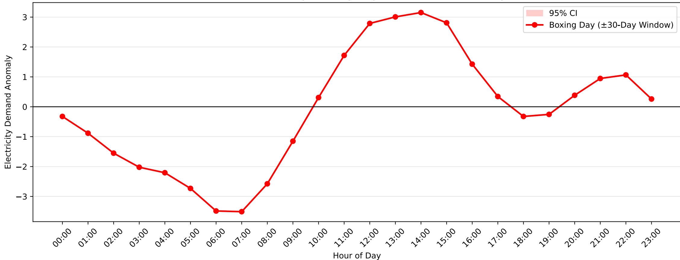
Mortdale Demand Anomaly: Boxing Day (2016–2017, \pm 30 -Day Window)
