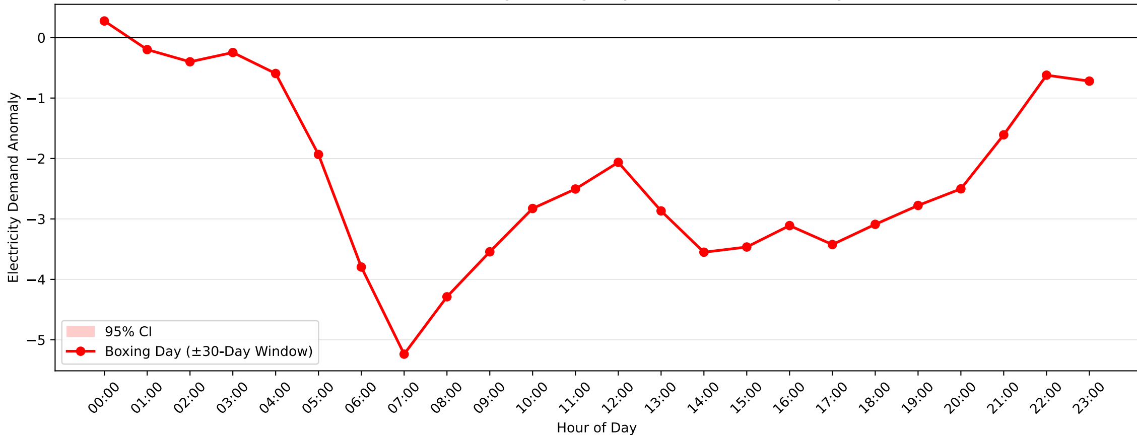
Mortdale Demand Anomaly: Boxing Day (2004–2005, \pm 30 -Day Window)
