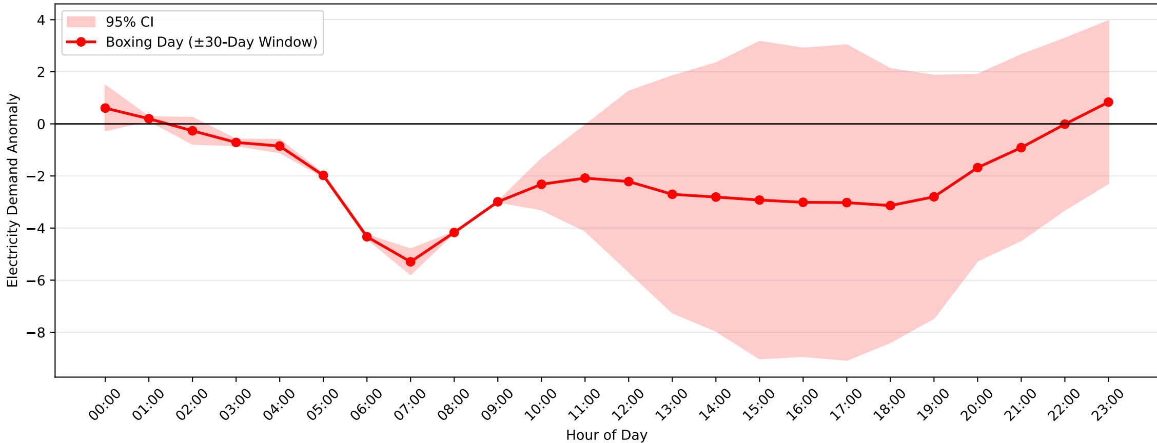
Mortdale Demand Anomaly: Boxing Day (2007–2008, \pm 30 -Day Window)
